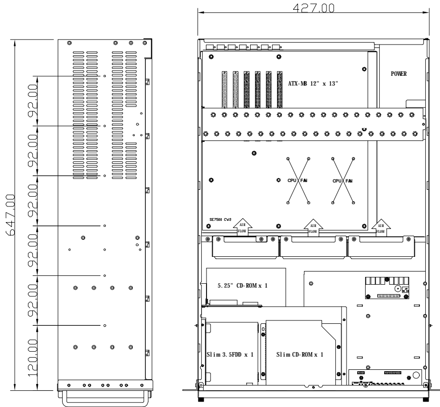
Left View
