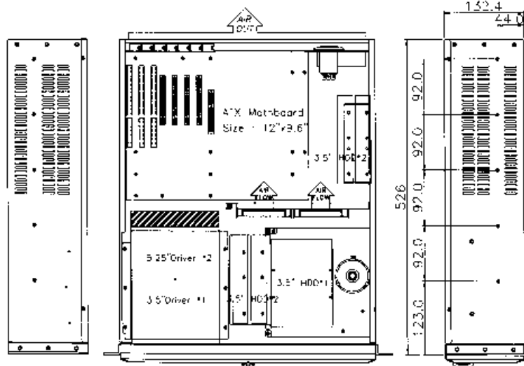
Left-side view
